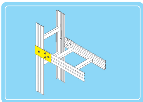
垂直分岐連接片 VERTICAL BRANCH PLATE
